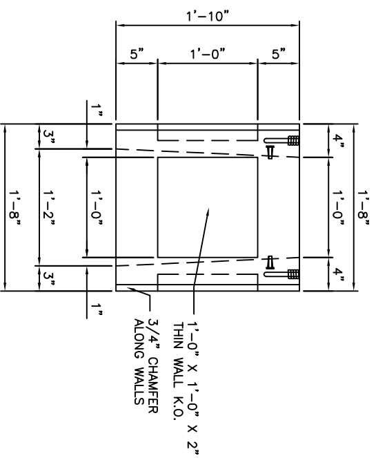
WALL B/D SCALE: 1 1/2" = 1'-0"
